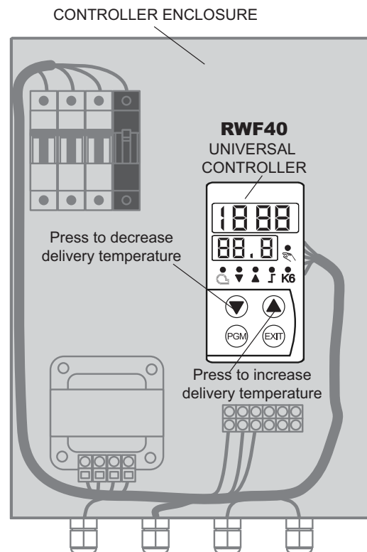
Figure 16a - Delivery temperature adjustment for Model: RWF40
