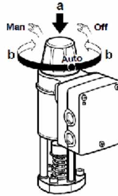
Figure 18 - Manual Control
