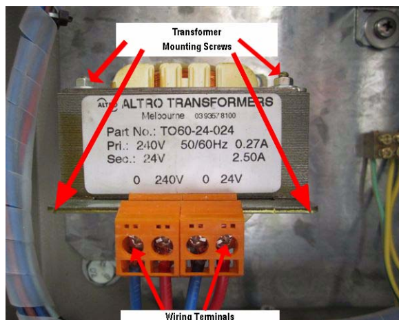
Figure 33 - Transformer
