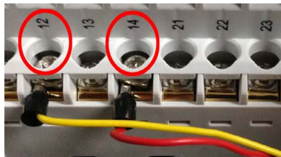
Figure 34b - 14 & 12 Terminals for RWF55.5
