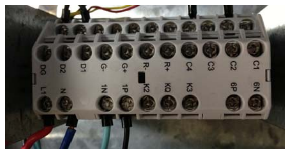
Figure 31b - Wire/Terminals
