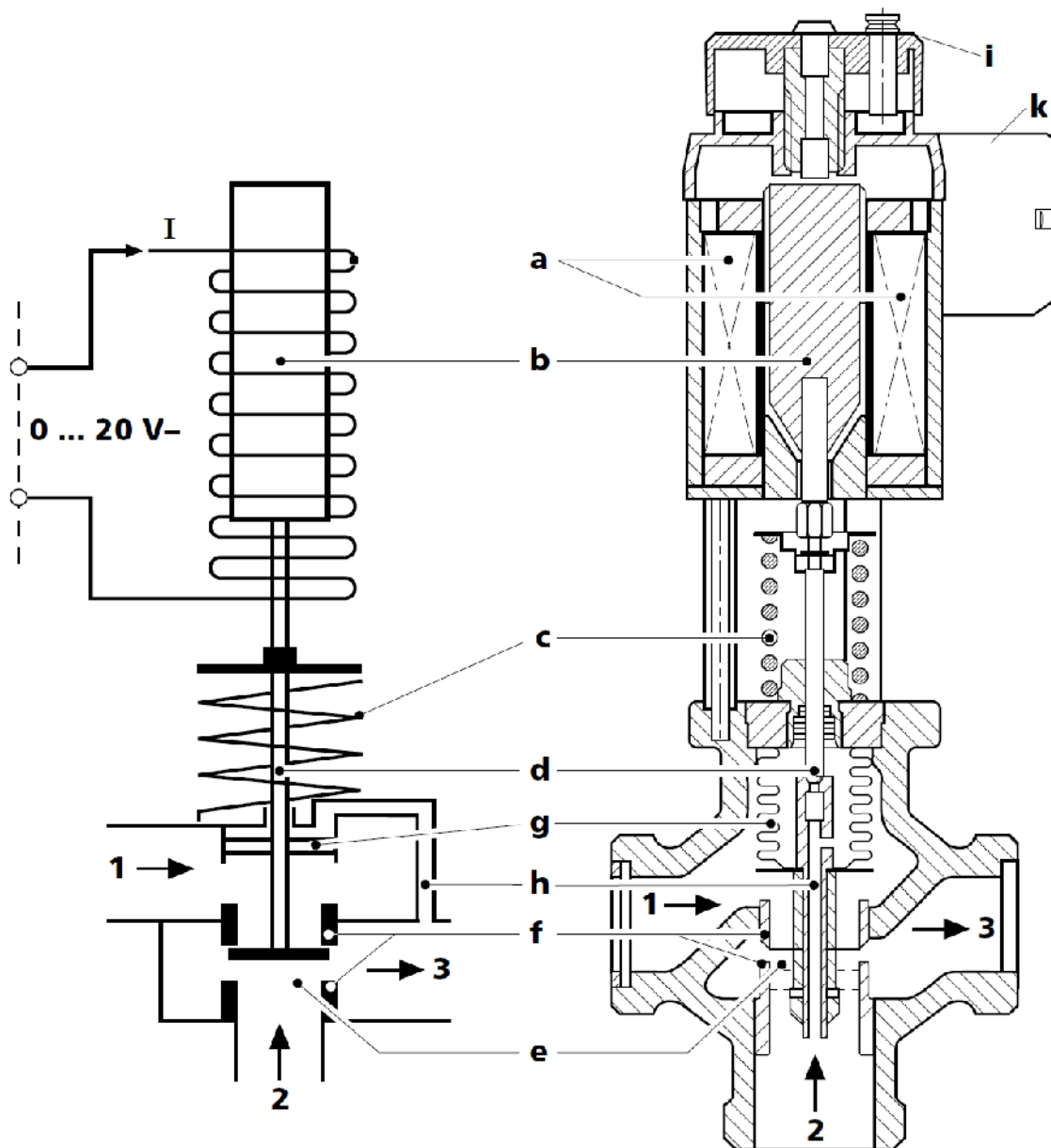
Figure 2 - Cutaway
