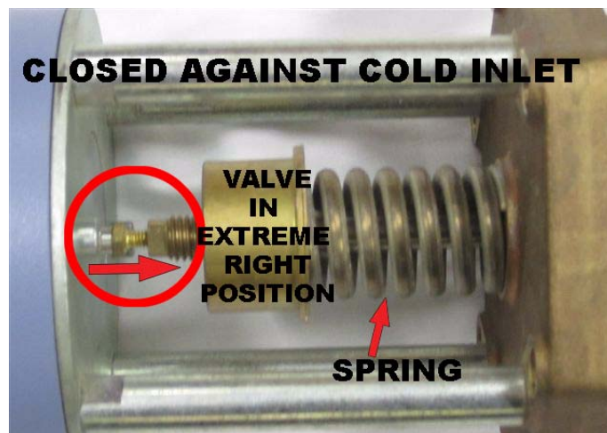
Figure 11 - Valve to extreme right - closed against Cold (10 Vdc)
