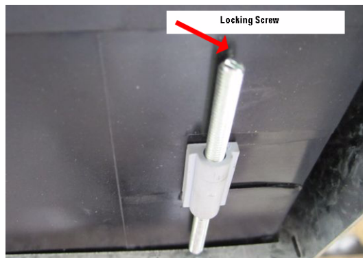
Figure 32 - Locking Screw
