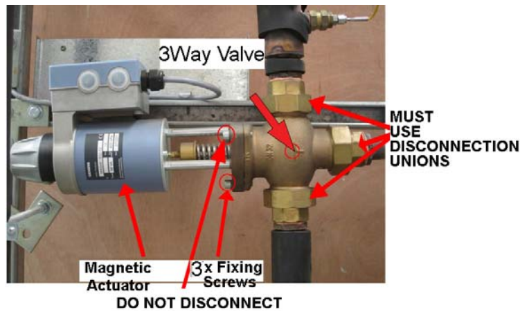
Figure 38 - 3 Way Valve Assembly
