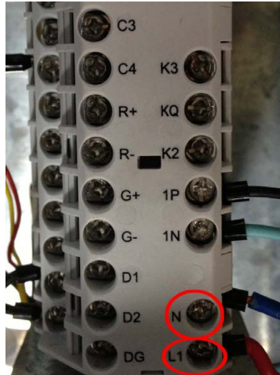
Figure 28b- Checking Power to Universal Controller
